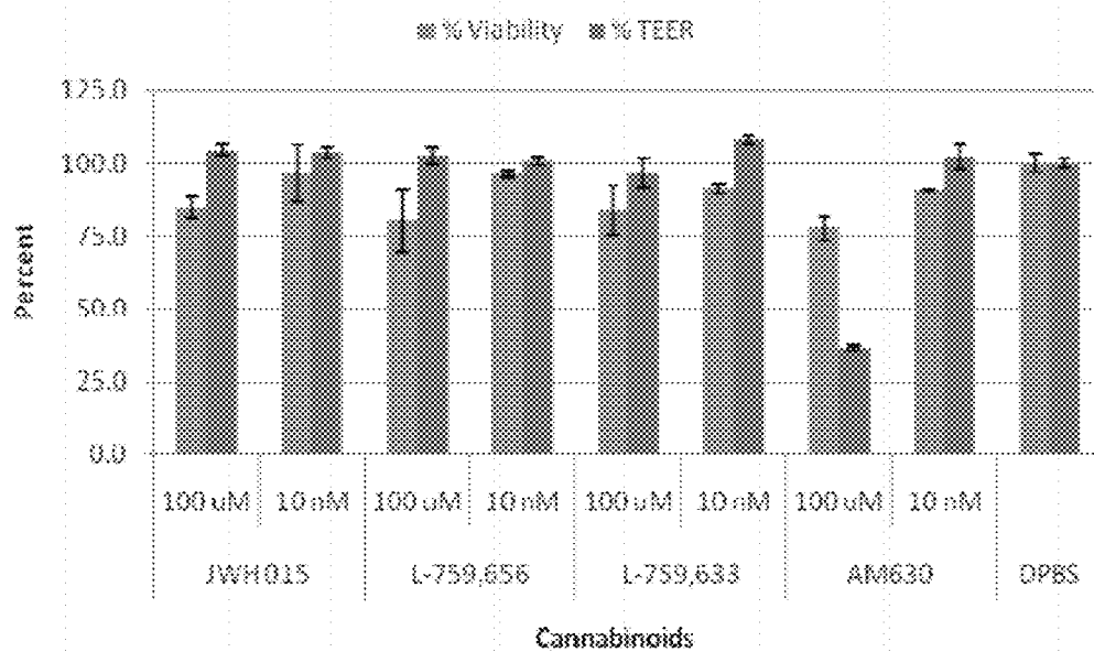
MTT VIABILITY AND TEER MEASUREMENTS FOLLOWING 7 DAY EXPOSURE OF THE TEST ARTICLES TO THE VEC-100 TISSUES (TEST ARTICLES WERE ADDED TO THE CULTURE MEDIUM).
